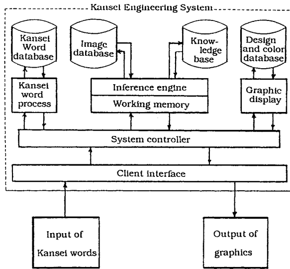
FIGURE 25.5 A system structure of the Kansei Engineering System.
